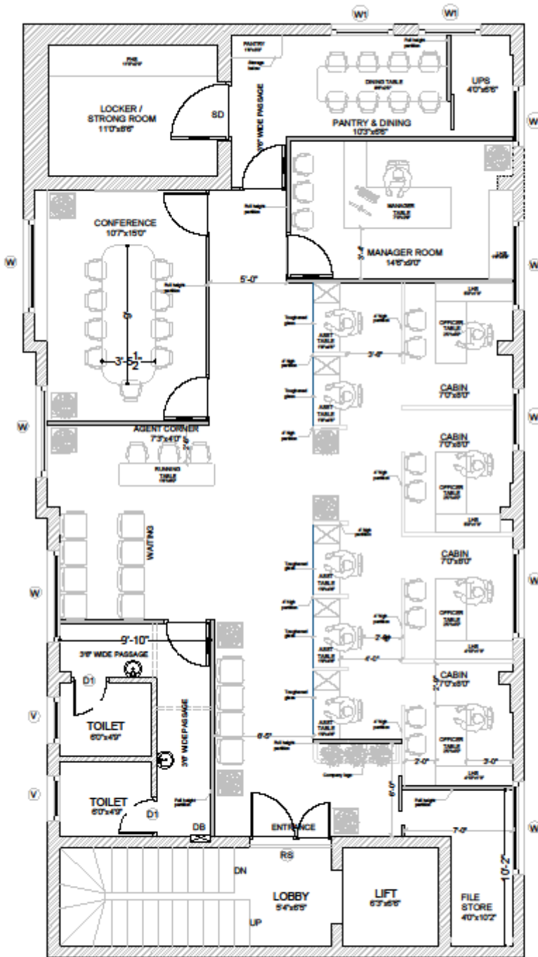
INTERIOR LAYOUT - FIRST FLOOR OPTION-8
